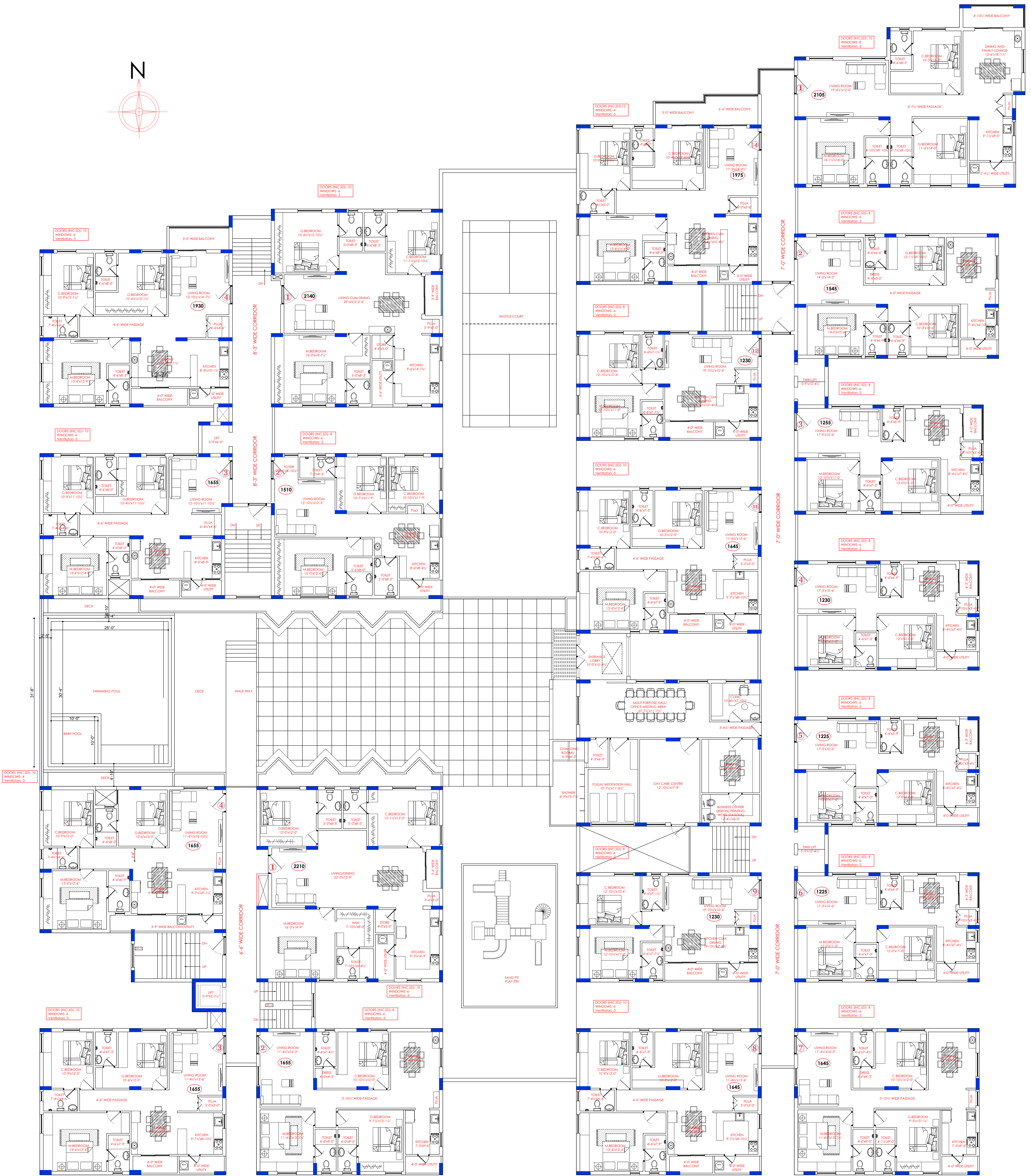
FIRST FLOOR PLAN
